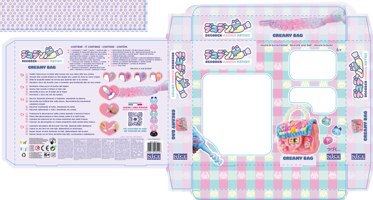
48510 MOMOMI DECODEN BAG DIMENSION: 31.1x25.3x5cm PRINT: 4C + GLOSSY FINISH magenta shape in "GLOSSY FINISH" level
